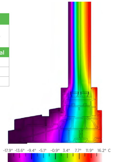
Design Advanced Slider – Sash Thermal Imagery
