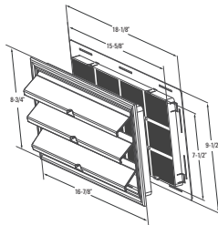
Gable Vent Cap installed with siding
